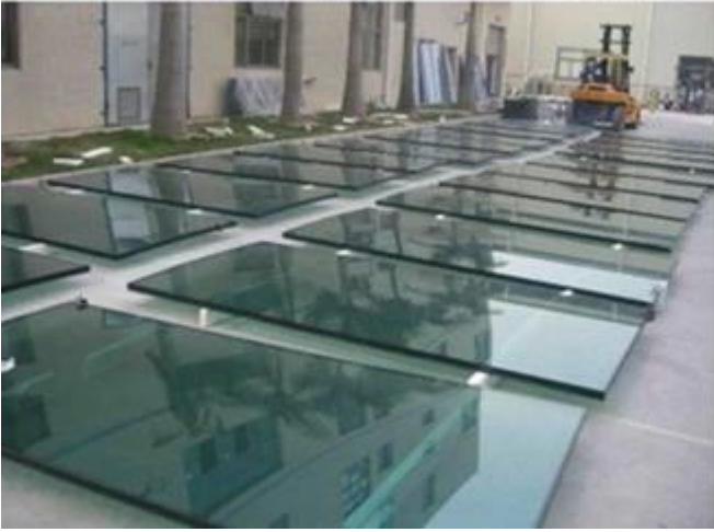
Tempered-laminated-reflective insulated glass :
