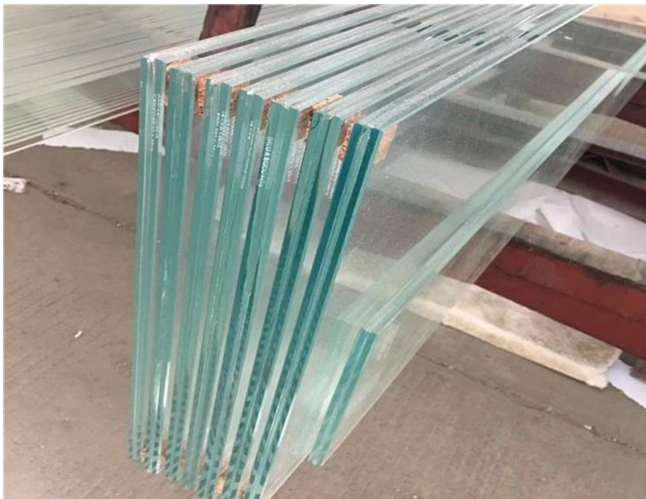
Professional production line for 5 + 5 mm ultra-clear tempered laminated glass
